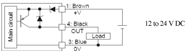
PNP Output Type
