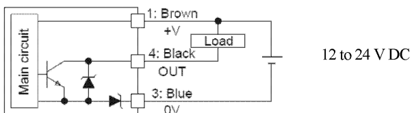
NPN Output Type
