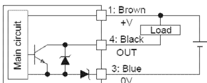
NPN Output Type
