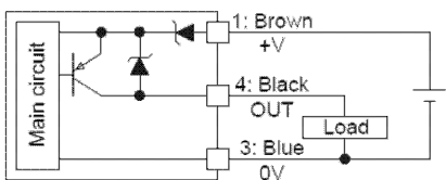
PNP Output Type
